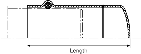
A half sleeve, on one side to slip over, other side with welded closing cap
