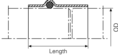
A half sleeve, on one side to slip over, other side to weld on with fillet weld
